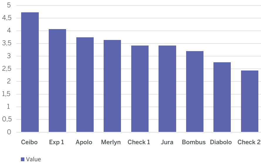
Growth Initial Score (Year 2017).
